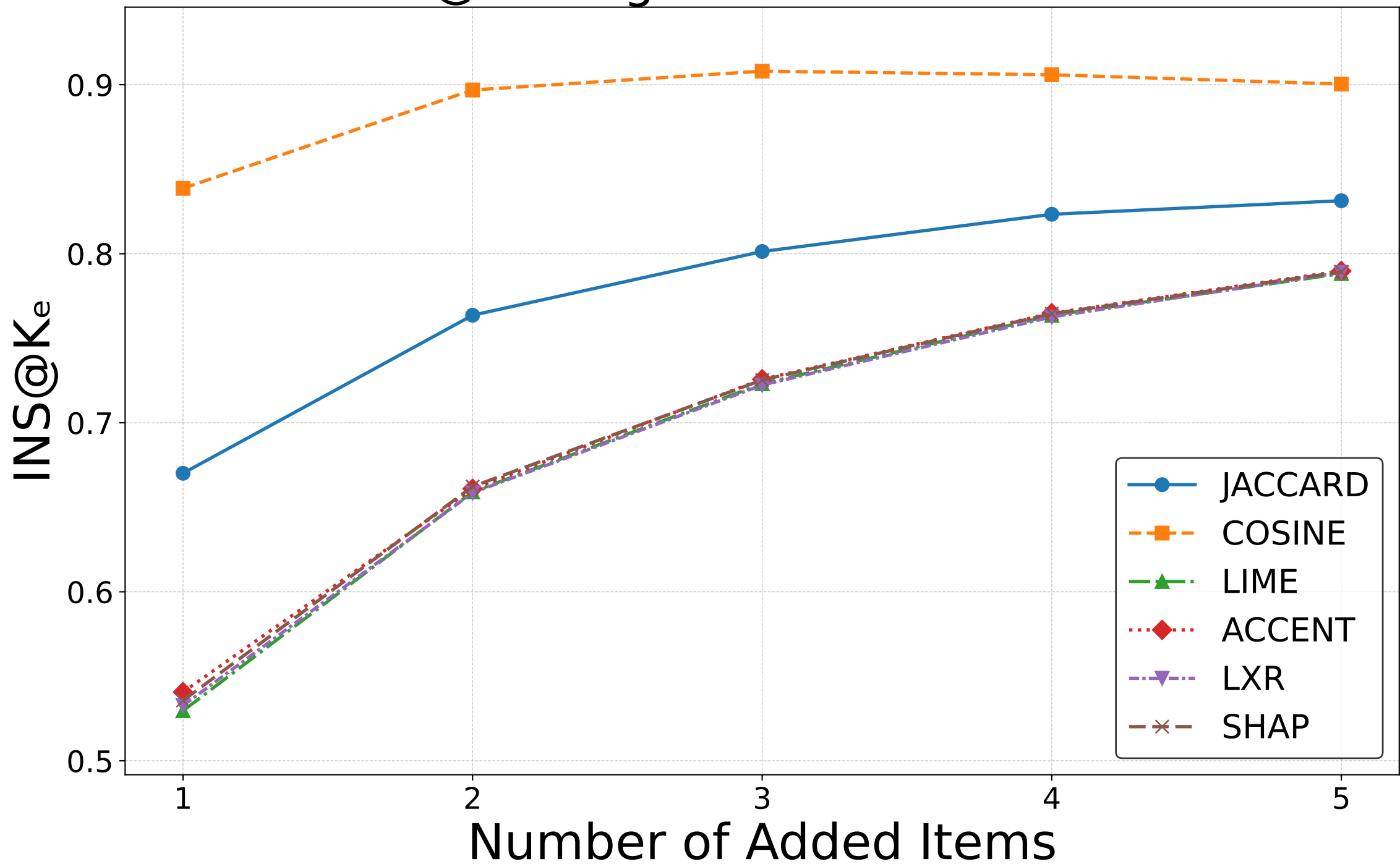
INS@Ke. Higher values are better
